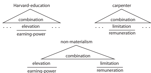
Figure 2: ‘Harvard-educated carpenter’.
