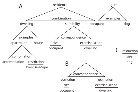
Figure 3: ‘Apartment dog’.
